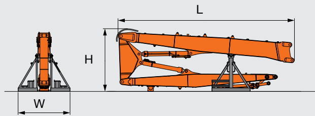
High reach demolition 25 m
