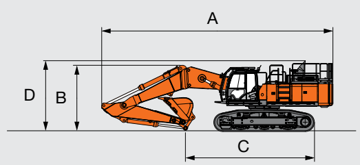
Mono block boom
