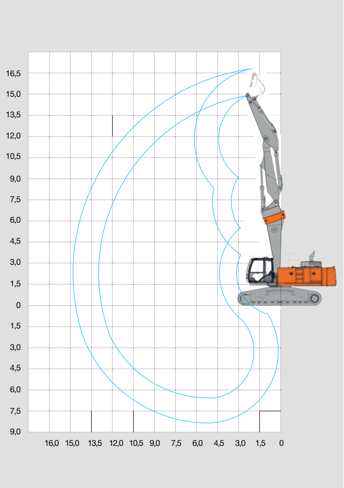
ZX600MC-7 2-Piece Demolition Front
