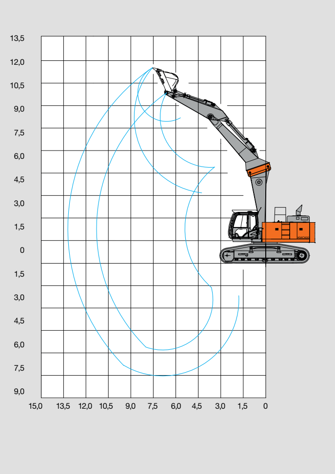
ZX600MC-7 Monoboom-Front
